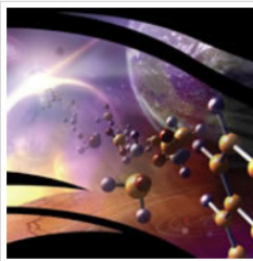
Astrobiology
