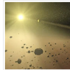
Cosmochemistry
